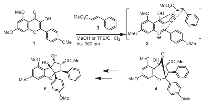
Figure 1. Photochemical cycloaddition of 3 and 3-hydroxyflavone 1 to access methyl rocaglate 5 .
