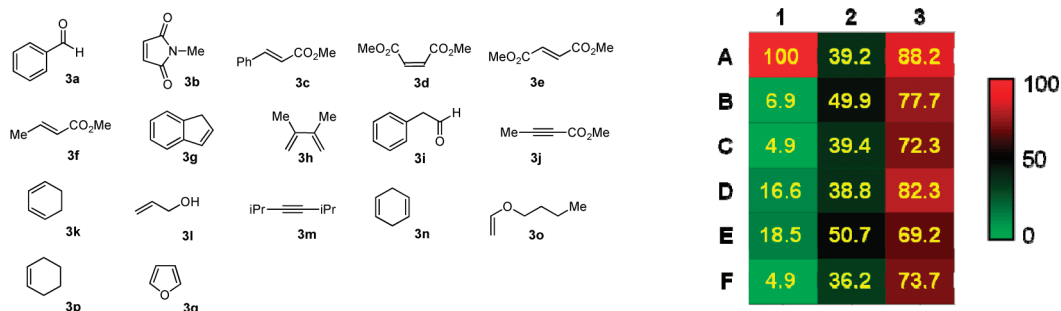
Figure 4. List of dipolarophiles used in fluorescence quenching and “heat map” of fluorescence measurements using a microplate reader. Fluorescence quenching data presented are an average of three data points 8 and have been normalized to a scale from 0 to 100%, where 100% represents the fluorescence emission of DMQ in the absence of dipolarophile. A1 represents the emission of 80 \mu M DMQ in 200 \mu L of dioxane: Fluorescence emissions reported in the presence of 0.05 M dipolarophile were normalized according to A1 . 3a : B1; 3b : C1; 3c : D1; 3d : E1; 3e : F1; 3f : A2; 3g : B2; 3h : C2; 3i : D2; 3j : E2; 3k : F2; 3l : A3; 3m : B3; 3n : C3; 3o : D3; 3p : E3; 3q : F3. Measurements were performed at an excitation wavelength of 350 nm and an emission wavelength of 470 nm with filter cutoff at 455 nm.
