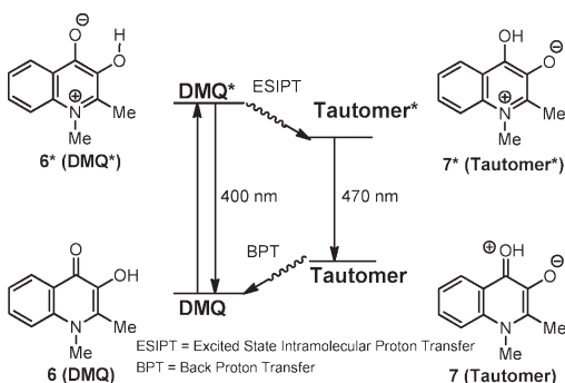
Figure 2. ESIPT of 3-hydroxyquinolinone 6 (DMQ).
